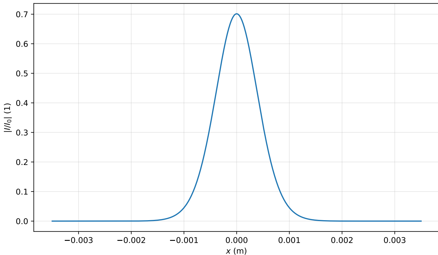
Intensity profile I(x, y = 0, z = 1.831m)/I_0 , P_{in}=0.3P_{cr} , artificial time
